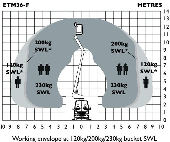
Platform mounted on a 5.2T GVW Iveco Daily 50C
