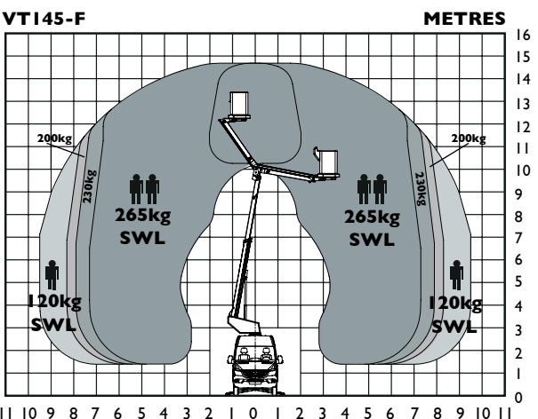
Working envelope at 120kg, 200kg, 230kg & 265kg bucket SWL
