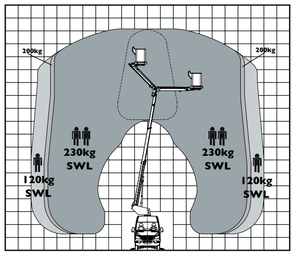
Working envelope at 120kg, 200kg & 230kg bucket SWL
