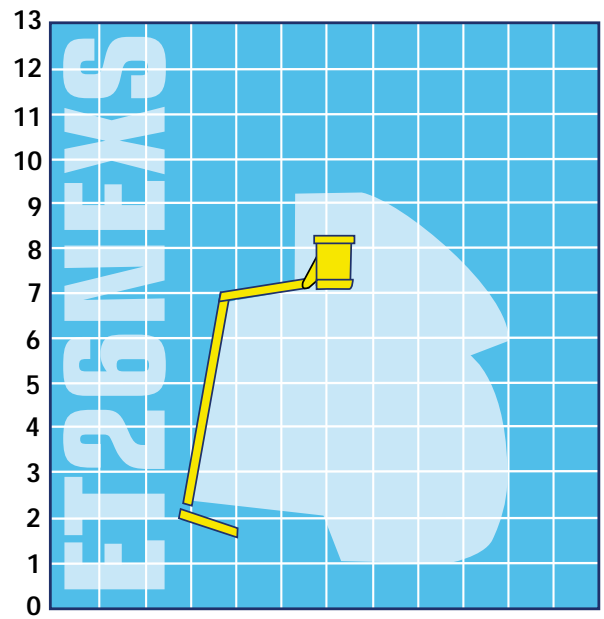
All dimensions in metres Reach of ET26/30NEXS
